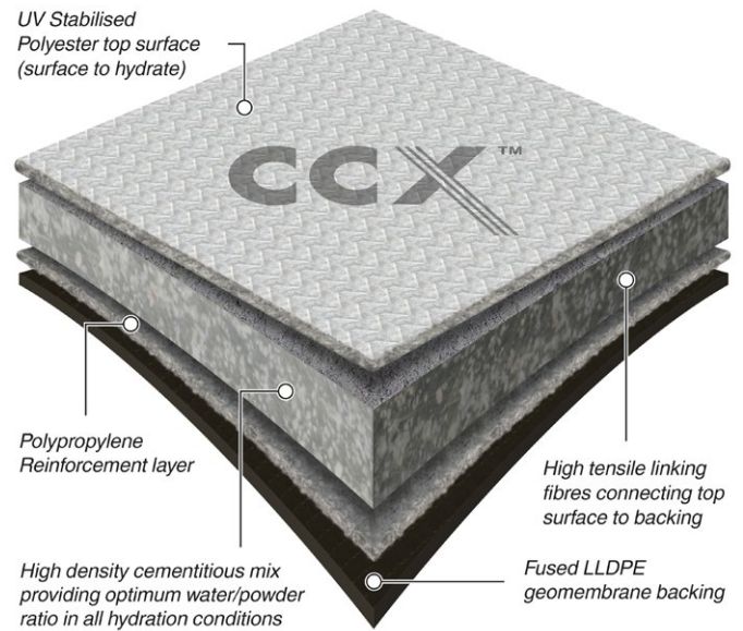
Typical CCX™ cross section
