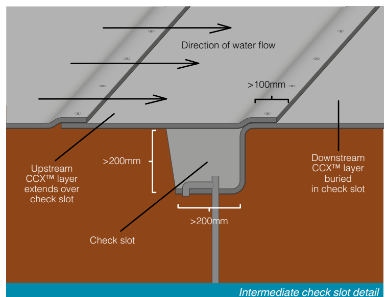
Intermediate fixings for profiling
