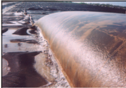
Water draining from a Geotube® container.
